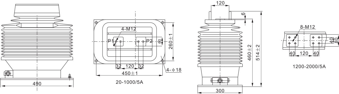
LZZB9-35D Overall Dimension
