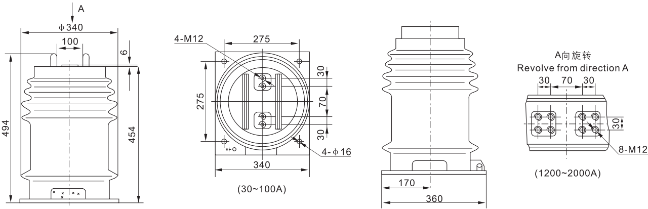
LZZB9-35C Overall Dimension
