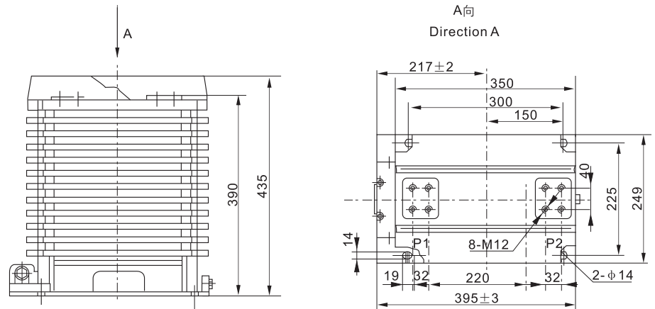
LZZBJ9-36/250W1(1500-2500A) Overall Dimension
