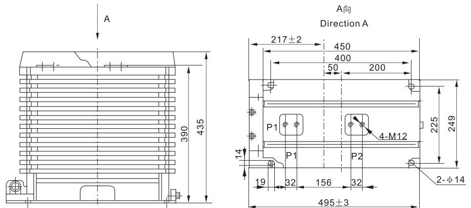
LZZBJ9-36/250W2(20-1250A) Overall Dimension
