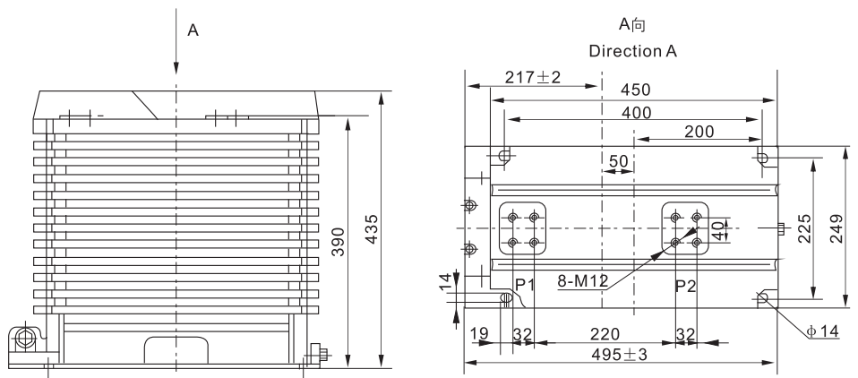
LZZBJ9-36/250W2(1500-2500A) Overall Dimension
