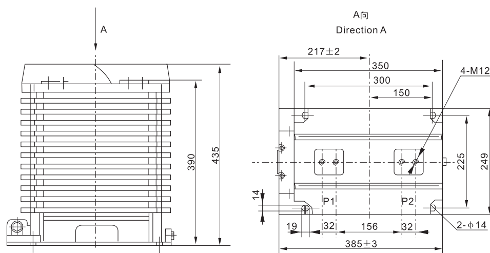
LZZBJ9-36/250W1(120-1250A) Overall Dimension
