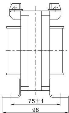
JDG4-0.5 Overall Dimension
