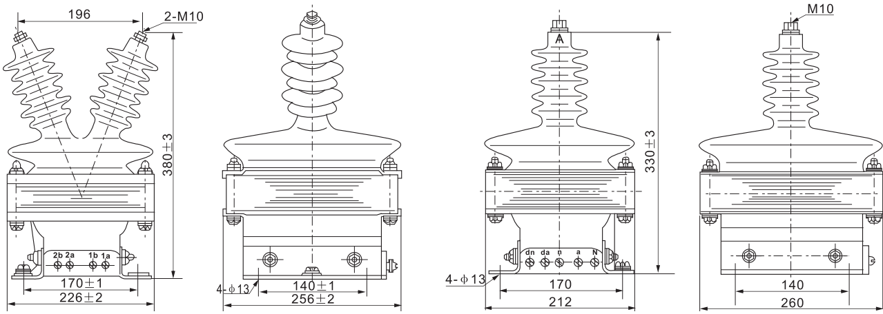
JDZ-15 Overall dimension
