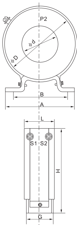
RCT Overall Dimension
