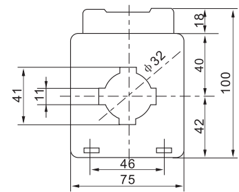
200/5A-600/5A
