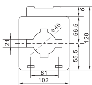
400/5A-1200/5A
