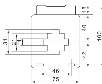
30/5A-300/5A(30/5-50/5A.2T)
