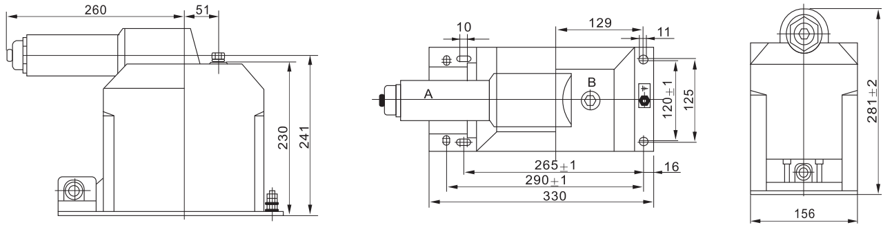
JDZR8-10A Overall Dimension
