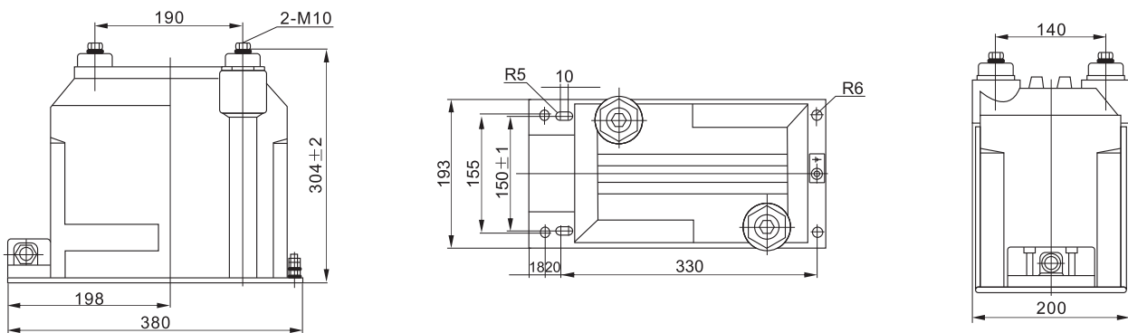
JDZR8-10C Overall Dimension
